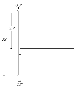
Offset Bracket
